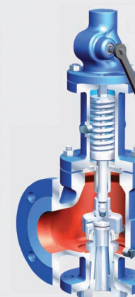
Safety Valves ASME Code Section VIII - Division 1 UV - Stamp NB - Stamp to AP1526.
