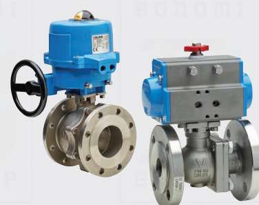
Electrically and Pneumatically Actuated Stainless Steel Ball Valves, Full Bore, Split Body Type. Direct Mount.
