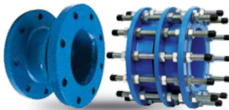
SERIES 44A DISMANTLING JOINTS. Collar made of St. Steel AISI 304 or Ductile Iron GJS500. Steel Flanges & Ductile Iron GJS500. PN 10/16 from DN 40 to DN 1600. Flanged Ends DIN PN 10/16.
