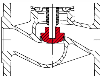
Screw down non-return regulating plug with marginal seat 1) (Set pressure refer to annex: Flow diagram)
